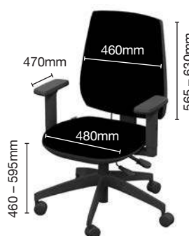
Salhouse Chair, Upholstered Back
